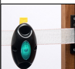
Voltage Indicator Flashes to indicate the fence is operating at an effective level. Stops flashing when voltage drops below 3kv. £30.00
